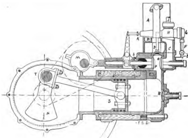
FIG. 324.—Roots' Kerosene Oil Motor for Vehicle Use. Sectional view showing the hot tube ignition, oil, vapor and air inlet and reciprocating parts. A is the vaporizing chamber surrounding the chimney of the hot tube, D. The eccentric, M, on the cam shaft actuates the exhaust valve, P, held in place by the spring, L, at the same time moving the link, K, which opens a valve contained in H, allowing a small amount of oil to be sprayed through the tubes, E, F, G, into the circulating chambers contained around the hot tube, D, as shown at B. The oil circulating around the heated space is transformed into vapor, which is fed into the channel, C, behind the inlet valve, O, which is opened by compression of its spring at the suction stroke. The valve, R, controlled by an adjustable compression spring, also admits sufficient air into the cylinder to give a mixture of the required proportion. The reciprocating parts are the piston, S, the connecting rod joined by a strap, T, to the crank pin, opposite to which is the balance weight, N. This section very well illustrates the workings of the type of explosive motor using hot tube ignition.
